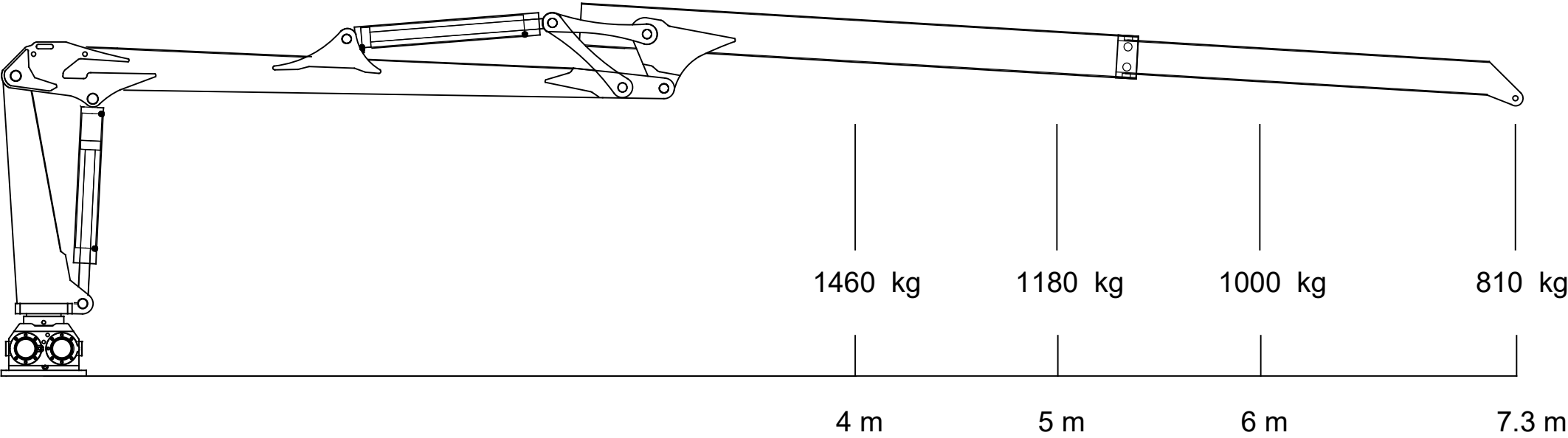
MTM 7300 lifting diagram
